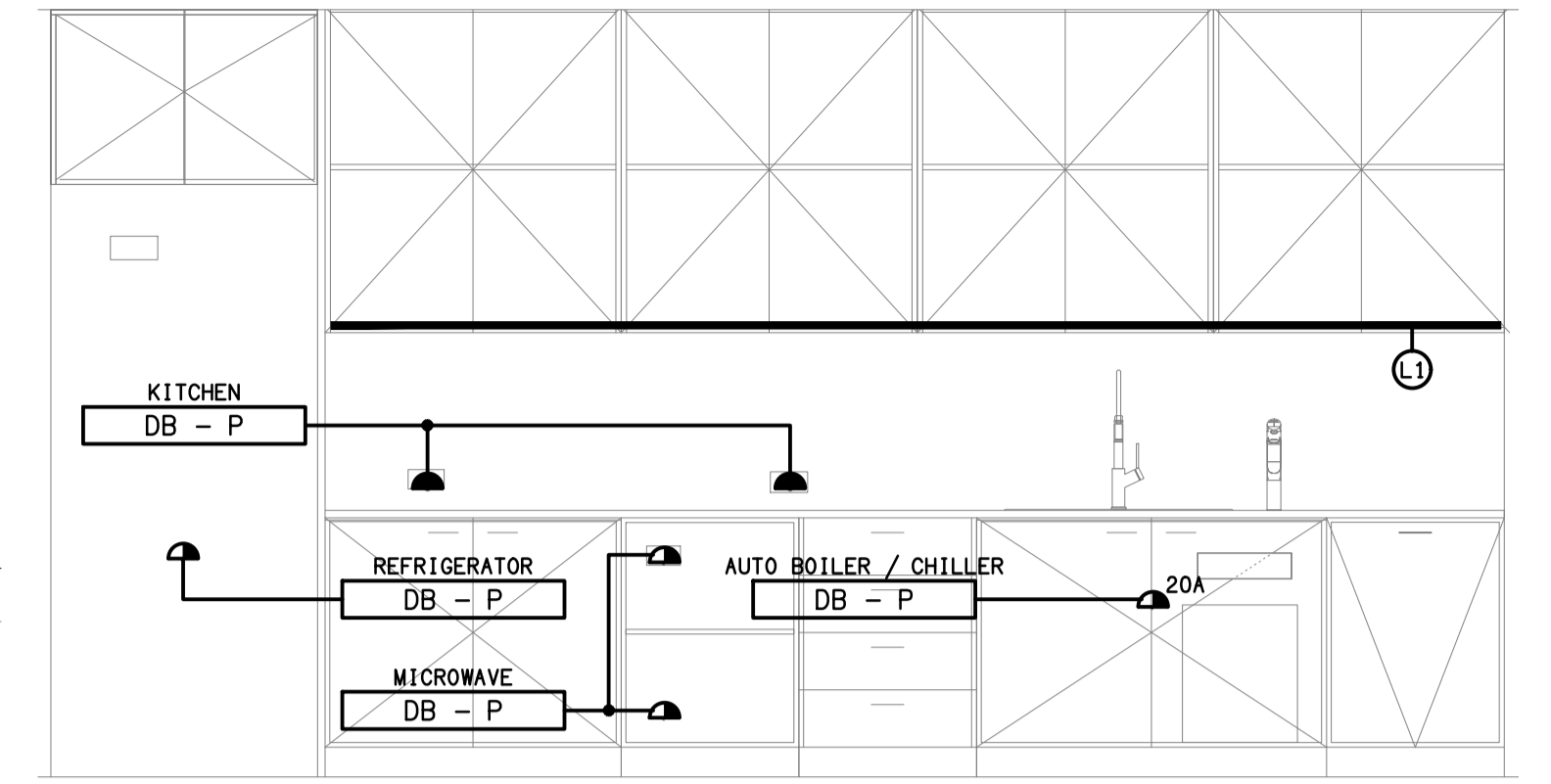
DETAIL A STAFF KITCHENETTE ELEVATION SCALE 1:25
